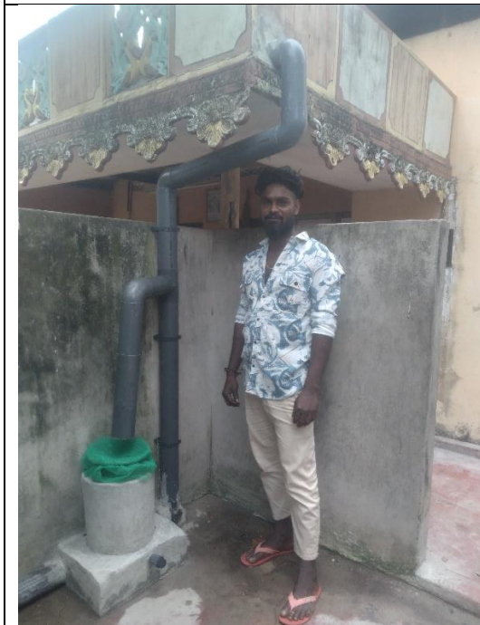
Thevaranjan Kantharaj well and well recharge system
