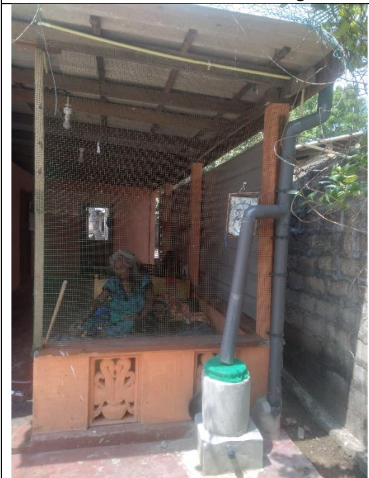
Thusyanthan Renuka well and well recharge system
